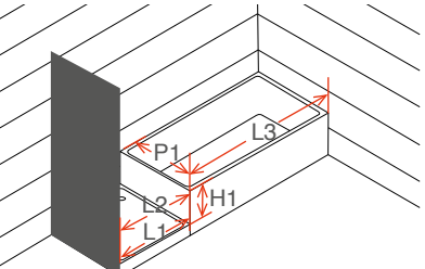
Base entre quatro paredes Showertray between four walls Receveur entre 4 murs
