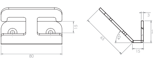
Cabide Duplo Alumínio Double Aluminium Hook Ref. 1603
