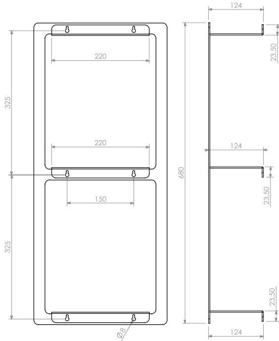
Prateleira Tripla Mate Alumínio Aluminium Triple Shelf Ref. 1611
