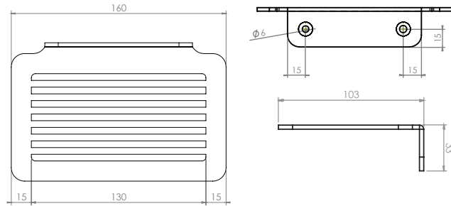
Saboneteira Alumínio Aluminium Soap Holder Ref. 1604
