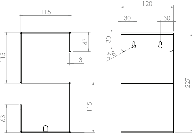
Porta Rolos Alumínio Aluminium Toilet Paper-holder Ref. 1608
